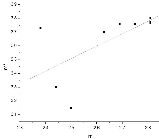
Figure1. Regression of mean crowding ( m^* ) on mean density ( m ) in P. nebulus population. M^*=1.69+0.74m , P<0.01
