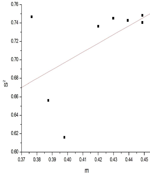
Figure2. Regression of variance ( S^2 ) on mean ( m ) in P. nebulus population (log scale). Y=0.3130+0.9636X , P<0.05
